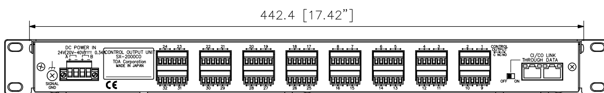
Rear View
